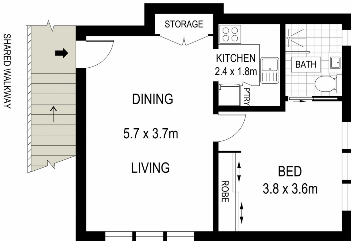
FIRST FLOOR
